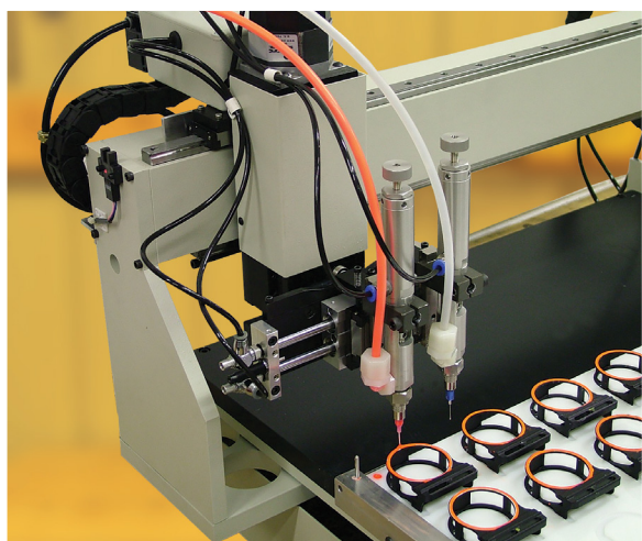
Automatic control and offsets for multiple valve/head combinations.
